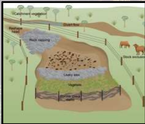
MERGE gully erosion model
