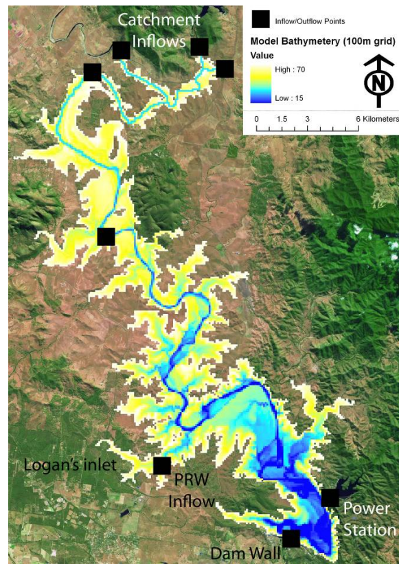
Figure 1. Lake Wivenhoe numerical model domain showing bathymetry (mAHAD) and inflow/outflow points.
