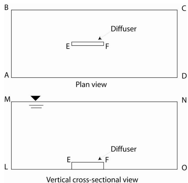
Figure 2. Near-field model domain showing (a) plan view and (b) vertical elevation. Length AB = 60 , AD = 170 m, height ML = 12 m. The diffuser length (EF) is 22 m and distance LE is 50 m. The diffuser ports (located along EF) are 1.7 m above the base elevation LO . All boundaries were represented using a “slip” boundary condition with the exception of CD/NO which was represented with an open or symmetry boundary condition. The near-field ELCOM simulation represented MN as a free water surface.
