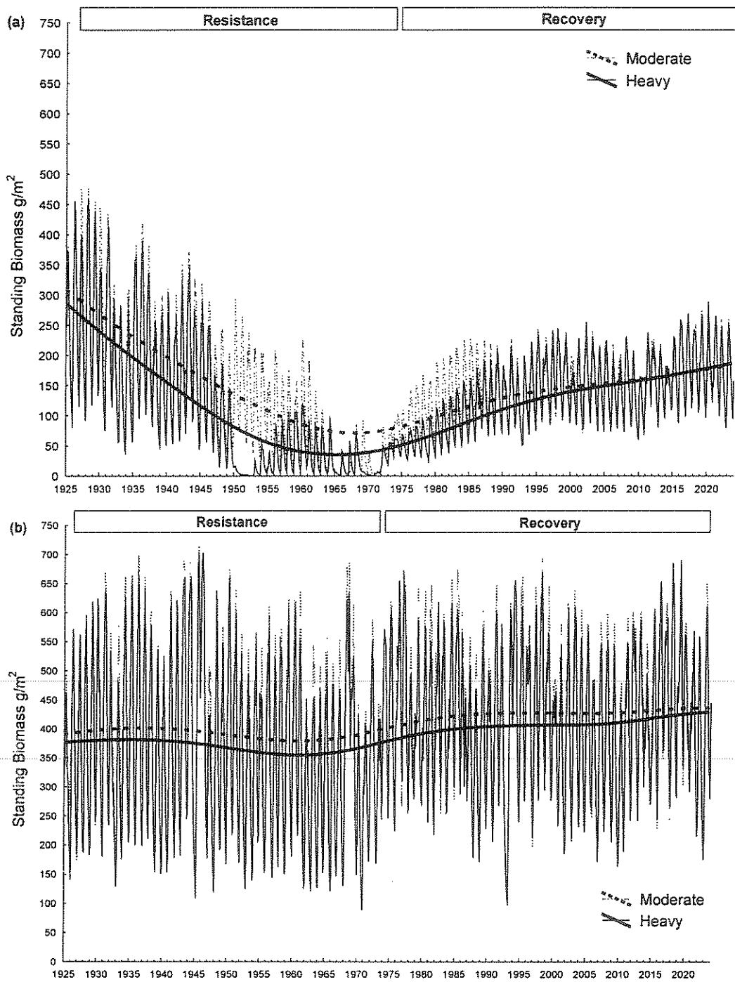
Fig. 6. SAVANNA model 100-year simulations of perennial grass biomass production for: (a) savanna woodland and (b) savanna grassland, first as impacted by moderate and heavy cattle grazing for a 50-year period to evaluate resistance, and then for a 50-year period without grazing to evaluate recovery .
