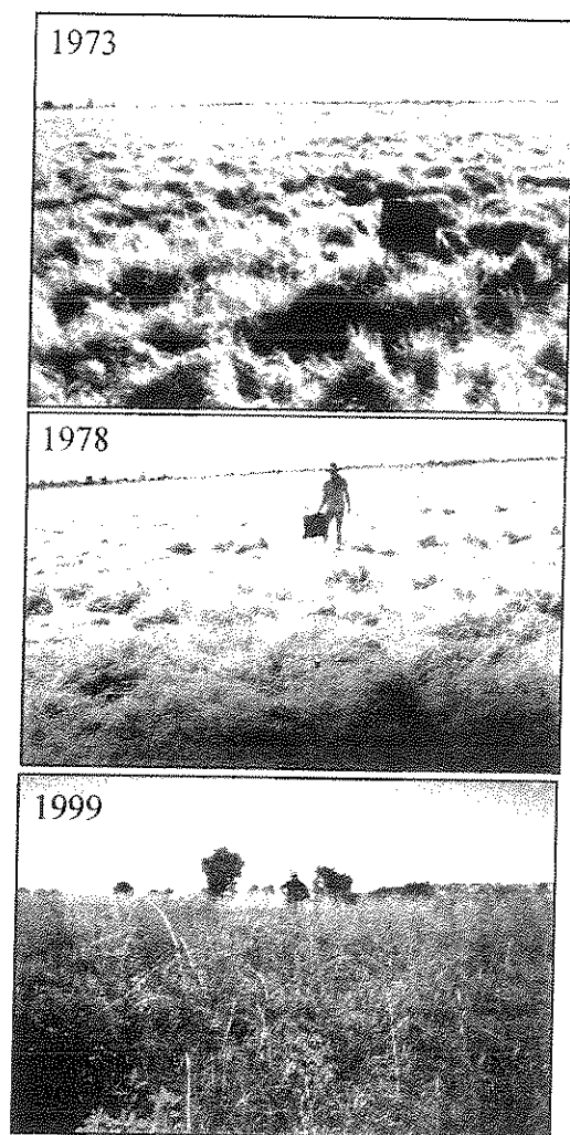
Fig. 5. Vegetation covers in 1973, 1978 and 1999 on a grey-clay grassland site.
