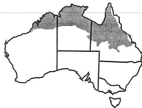
Fig. 1. Distribution of Australian savannas.
