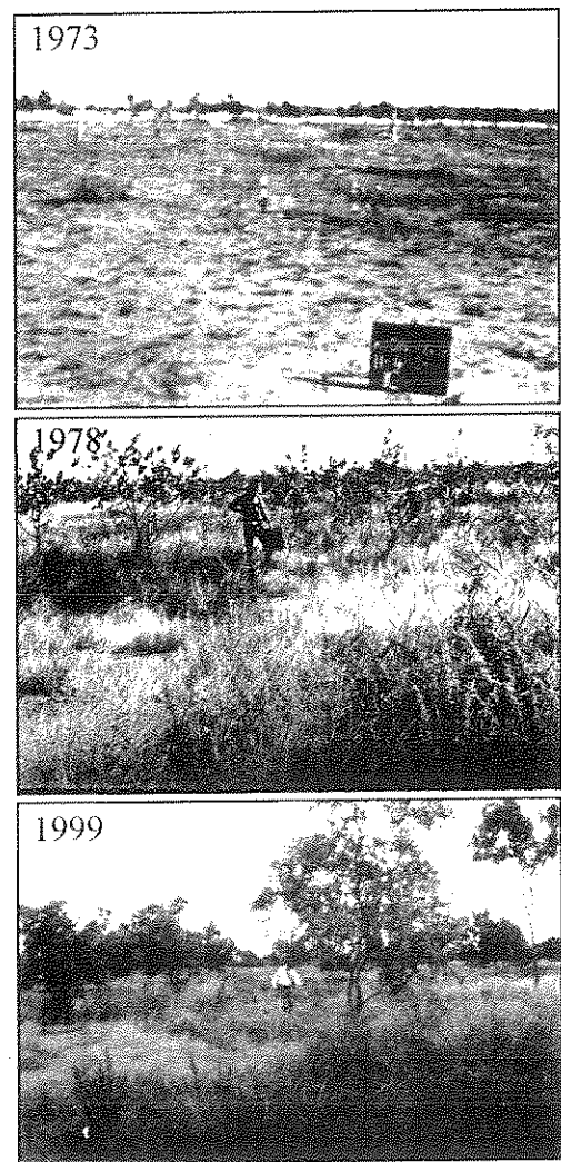
Fig. 3. Recovery of vegetation from 1973 to 1978 and to 1999 on a red-loam woodland site.
