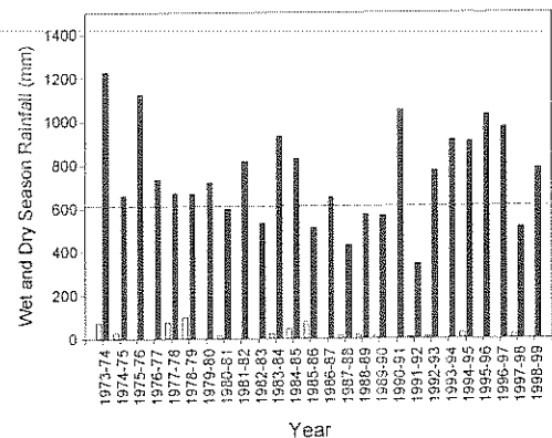
Fig. 4. Wet- and dry-season rainfalls for 1973 to 1999 relative to the wet-season mean of 617 mm. SAVANNA was driven by weather data from the VRD [Clewett et al 1994].
