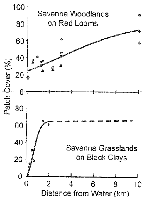
Fig. 2. Changes in the cover of perennial plant patches with distance from watering-points
