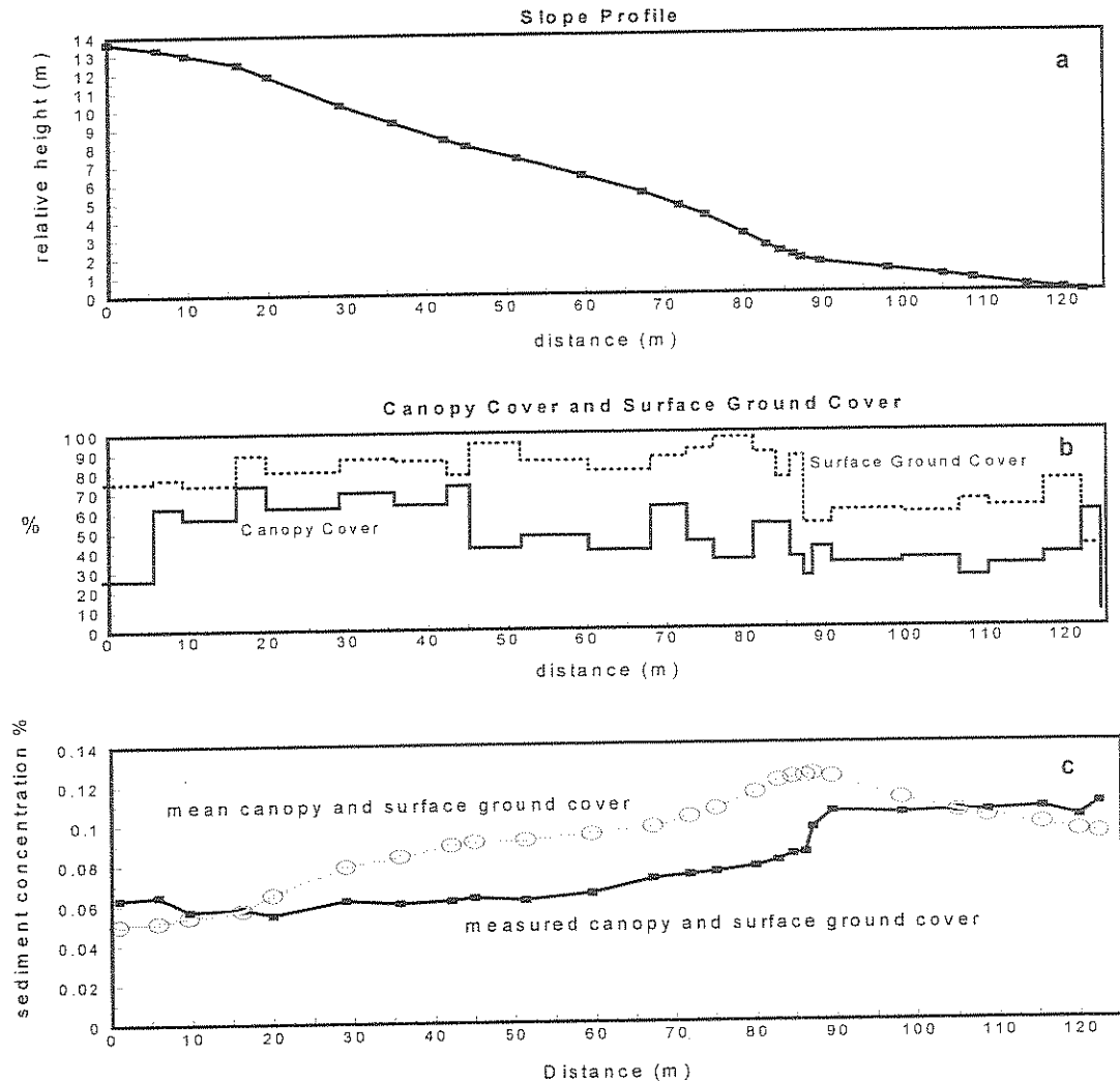
Figure 2. a) Representative hillslope profile, b) measured values of canopy and ground cover on the K2 watershed in July 1994, and c) simulated mean concentrations for both measured and average values of canopy and ground cover of the representative hillslope profile
