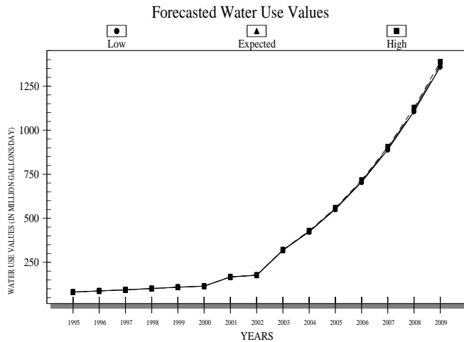
Figure 3: The Forecasted Domestic Water Demand, Equation 3
