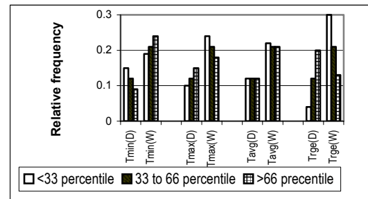
Tmin - Daily minimum temperature (°C); Tmax - Daily maximum temperature (°C) Tavg - Average of daily minimum and daily maximum temperature (°C) Trge - Range of daily minimum and daily maximum Temperature (°C) D - Dry state; W - Wet state
